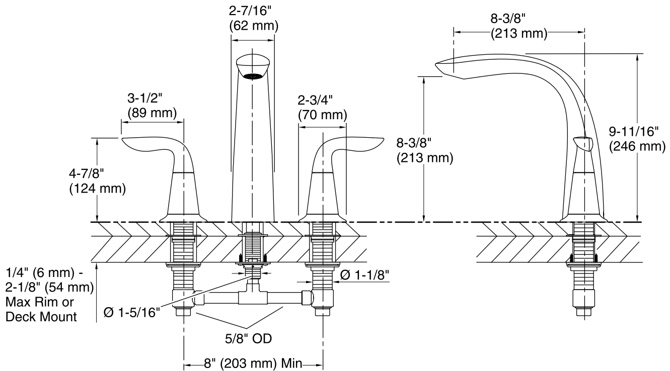
Rough + Finished Deck Mount Installation
