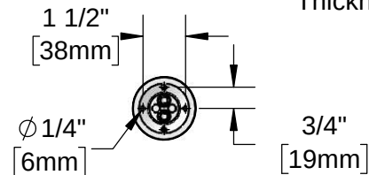
Bottom View VR Pin Hole Pattern
