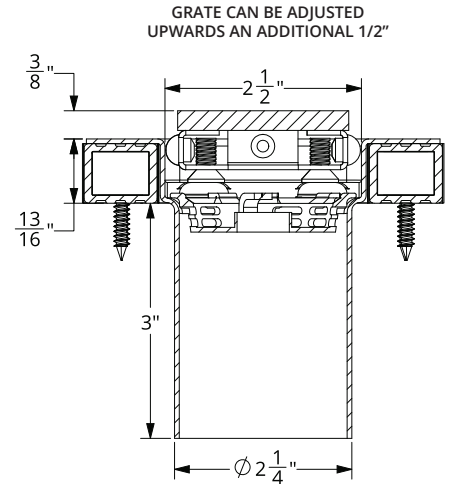
SECTION 1-1
