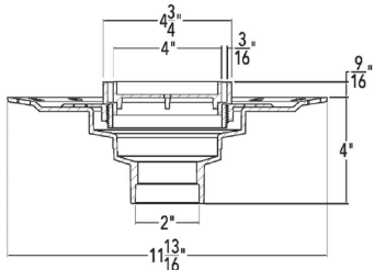
Section A-A RTDB 15
