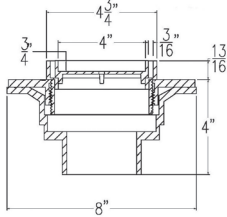
Section A-A RTD 15
