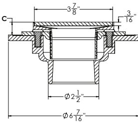
Section A-A 4" x 4" Center Drain
