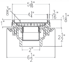
Section A-A LTD 5
