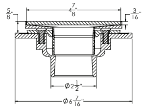
Section A-A 5" x 5" Center Drain
