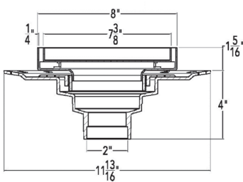
Section A-A TDB 20
