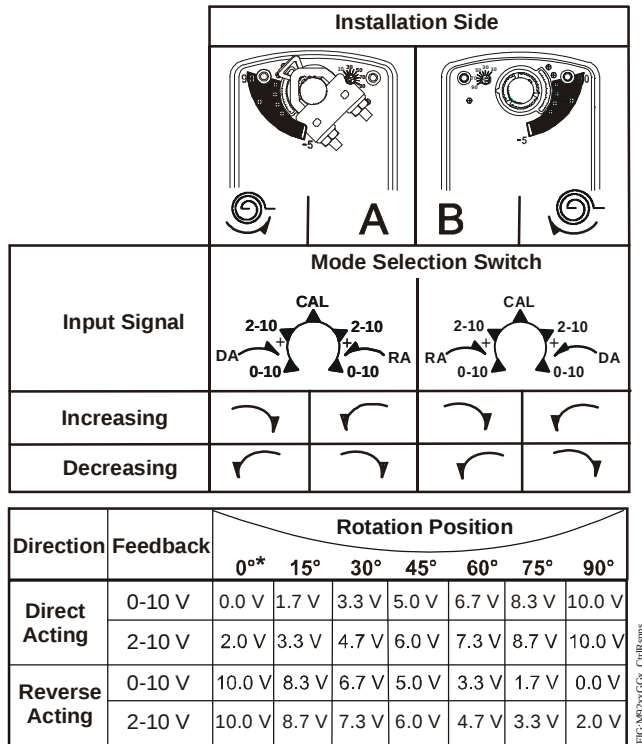
Figure 14: Control Response
