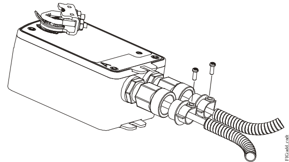
Figure 12: Adding Flexible Metal Conduit
