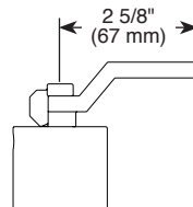
HL934-▲ Industrial Lever Handle
