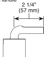
HL939-▲ Wire Handle
