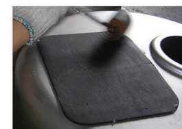
When applying the pad to the sink, a roller is used to flatten or even out the pad.
