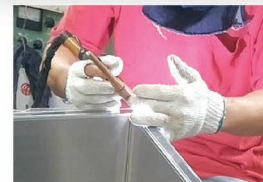
Butt Welding: the joints on the sink rim are butt welded.
