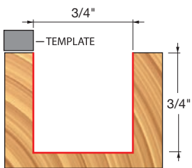
16-504 Top Bearing
