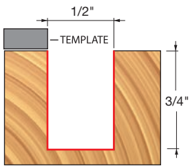
16-500 Top Bearing
