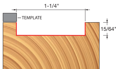
16-522 Top Bearing
