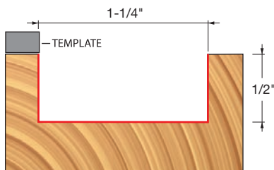
16-523 Top Bearing
