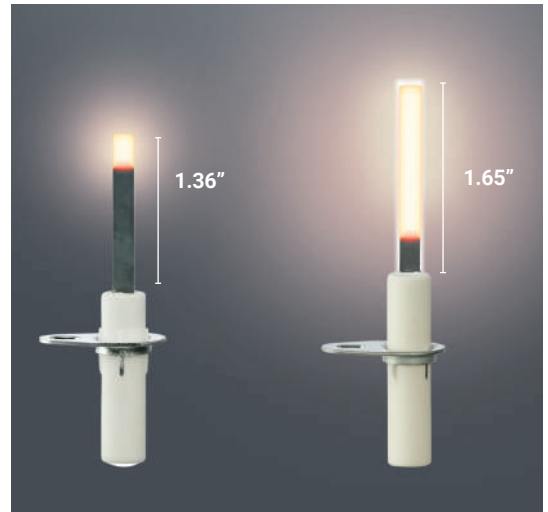
Glowfly® Igniter
