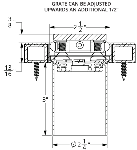
SECTION 1-1
