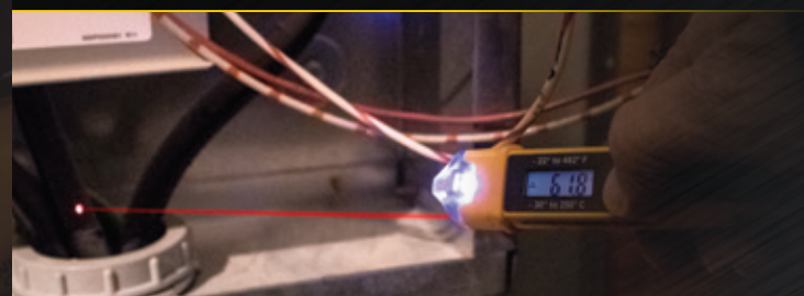
NCVT-4IR DETECTS: 12-1000V AC Designed specifically for HVAC applications. This 4:1 distance-to-spot ratio IR thermometer measures from -22 to 482° F (-30 to 250° C). Use convenient laser pointer to target measurement area for temperature measurement.
