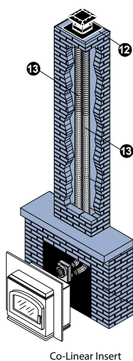
Co-Linear Insert
