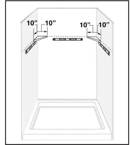
2. Using a level, mark 10" x 10" on each wall at determined height.
