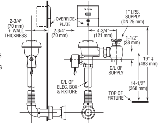
MODEL 140 ES-S
