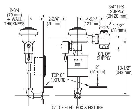
MODEL 195 ES-S
