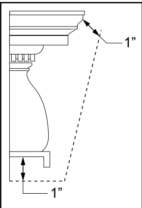
Figure 2.12 - A custom-formed mantel shield.
