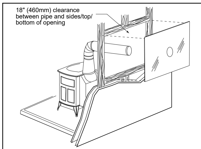
Figure 2.9 - An approved wall pass-through for Canada.
