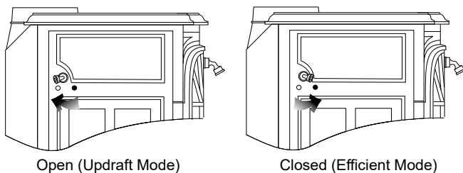
Figure 5.3 - The catalyst bypass damper is either open or closed. There are no intermediate positions.
