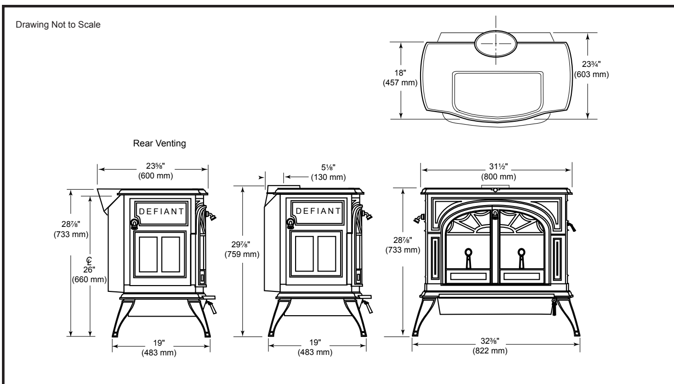
Fig. 1 Defiant 1975 dimensions.
