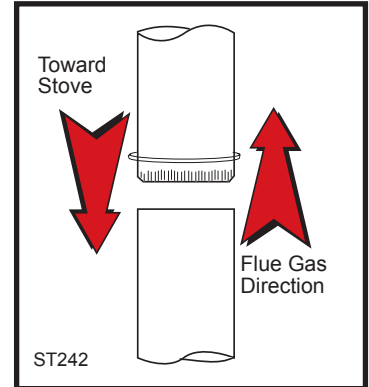
Fig. 5 Chimney connector.
